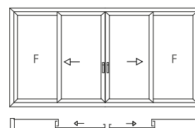
2 vie - 2 ante+2 fissi 2 rail-2 sash+2 fixed
