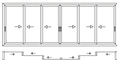
3 vie - 6 ante 3 rail-6 sash
